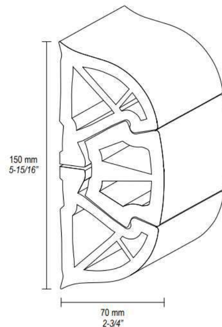
BUMPER 150
