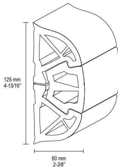
BUMPER 125
