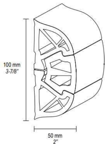
BUMPER 100
