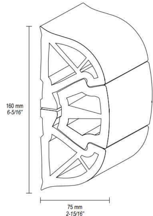
BUMPER 160
