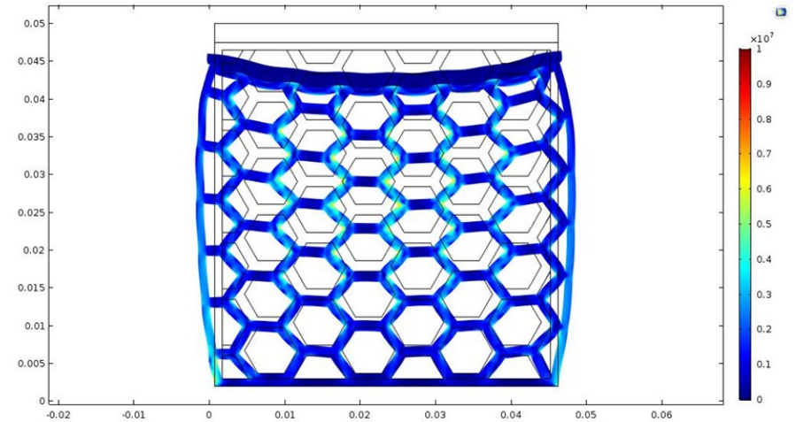
Von Mises stress 2D distribution map
