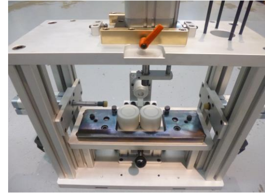
Test equipment brake calipers pression ◀ automotive industry. Components' construction and assembly.
