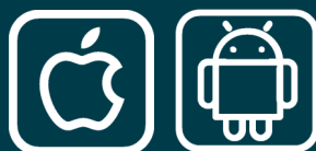
Cross-platform Application
