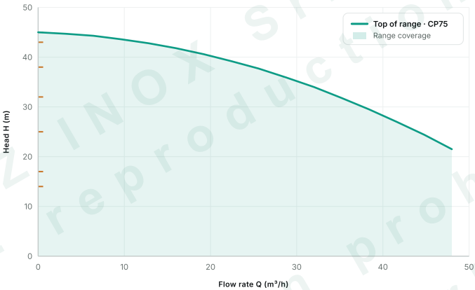
RANGE COVERAGE Q-H · 50 HZ
