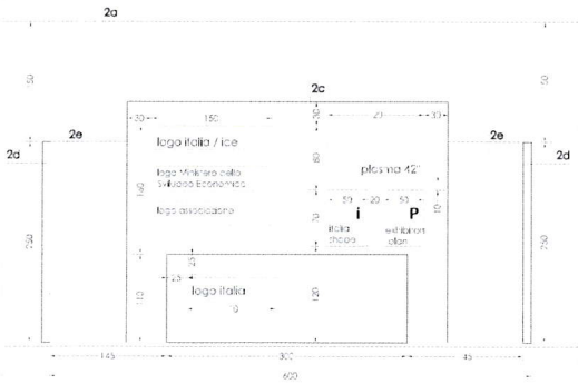
elevation solution2
