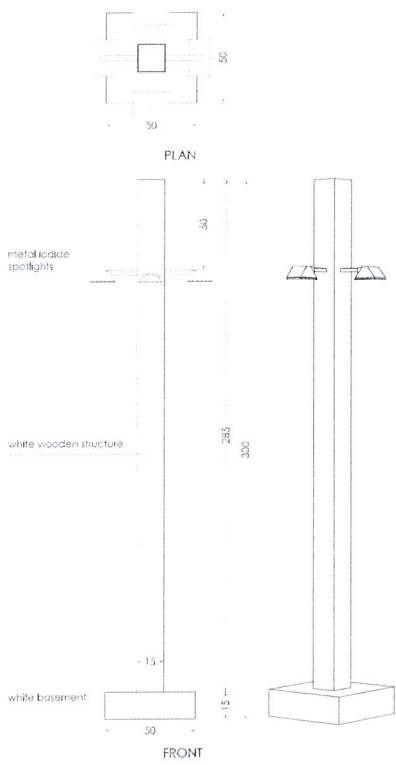
Lighting column
