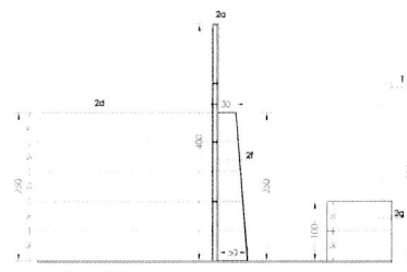
section E-E'
