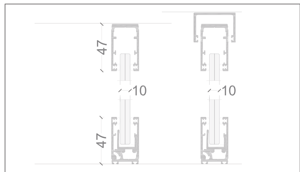
VERTICAL SECTION
