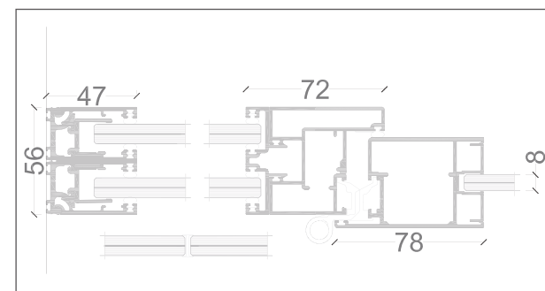
HORIZONTAL SECTION GLASS DOOR WITH FRAME
