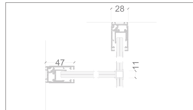
"T" JUNCTION
