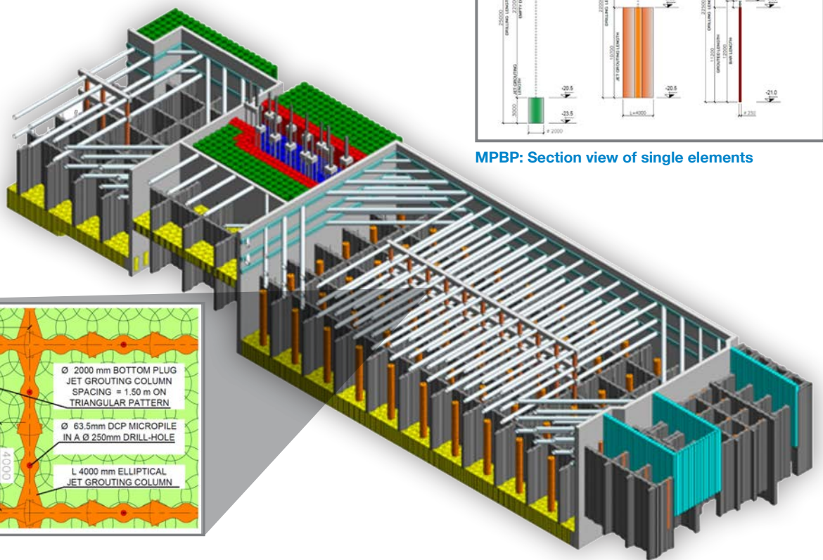
BIM of MPBP basic element
