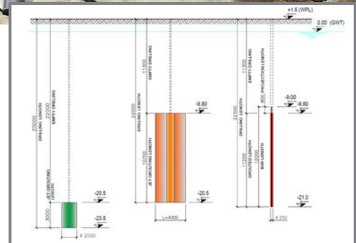
MPBP: Section view of single elements
