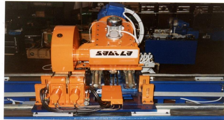
FLYING SAW CUT FOR WELDED TUBES
