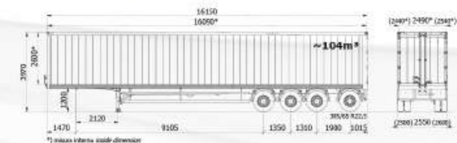
16.15m semi-trailer
