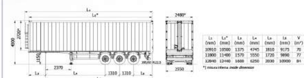
Short semi-trailer (10,5m - 11,5m - 12,5m)
