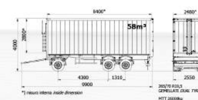
3-axle trailer
