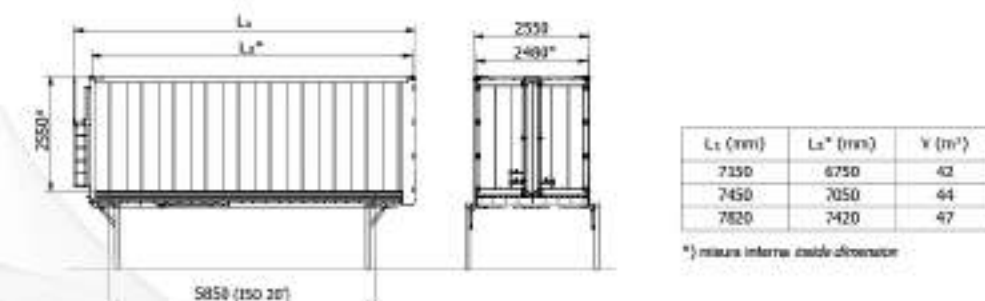
Swap body (closed case)
