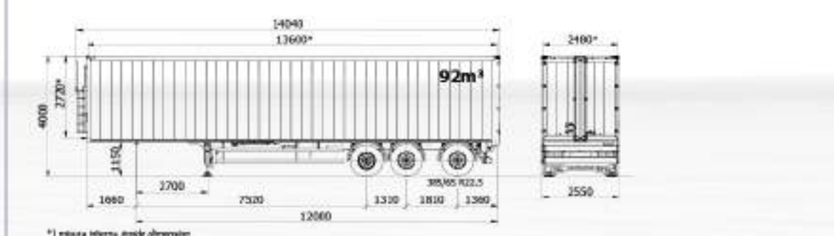
3rd axle rear semi-trailer
