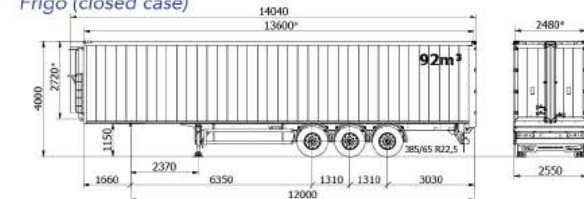
Frigo (closed case)
