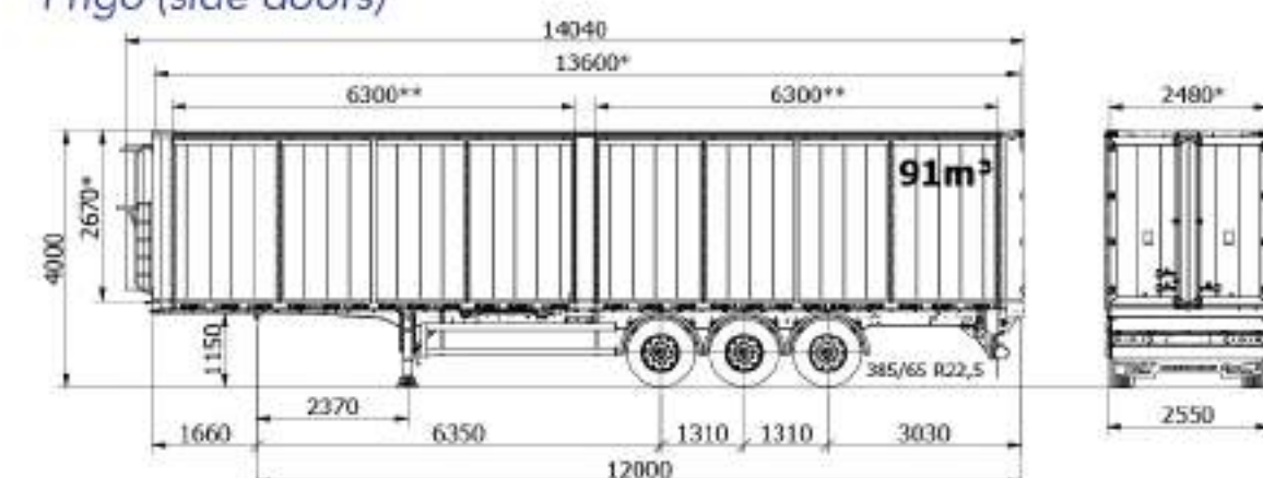
Frigo (side doors)
