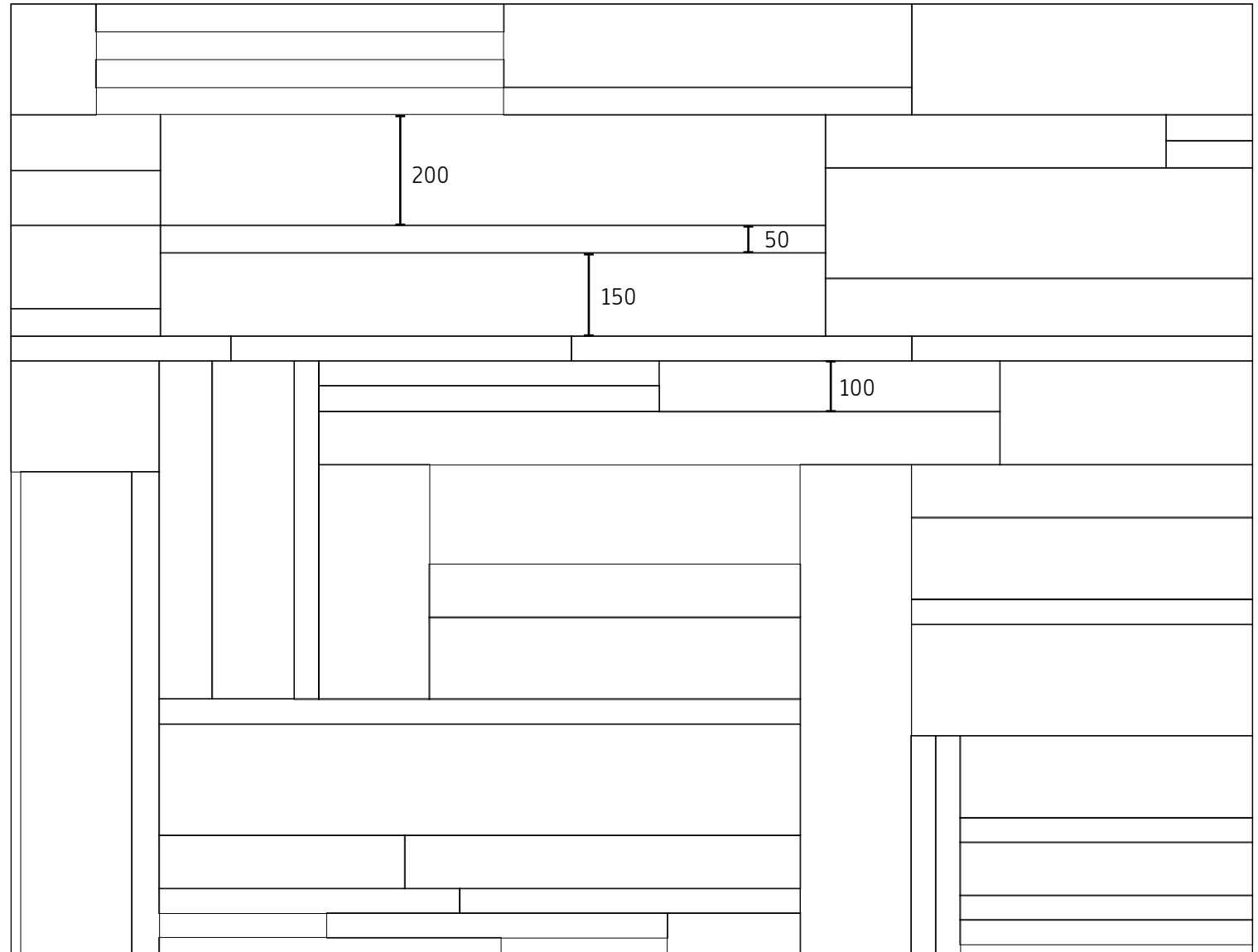
Mixed laying (mixed lengths and widths)
