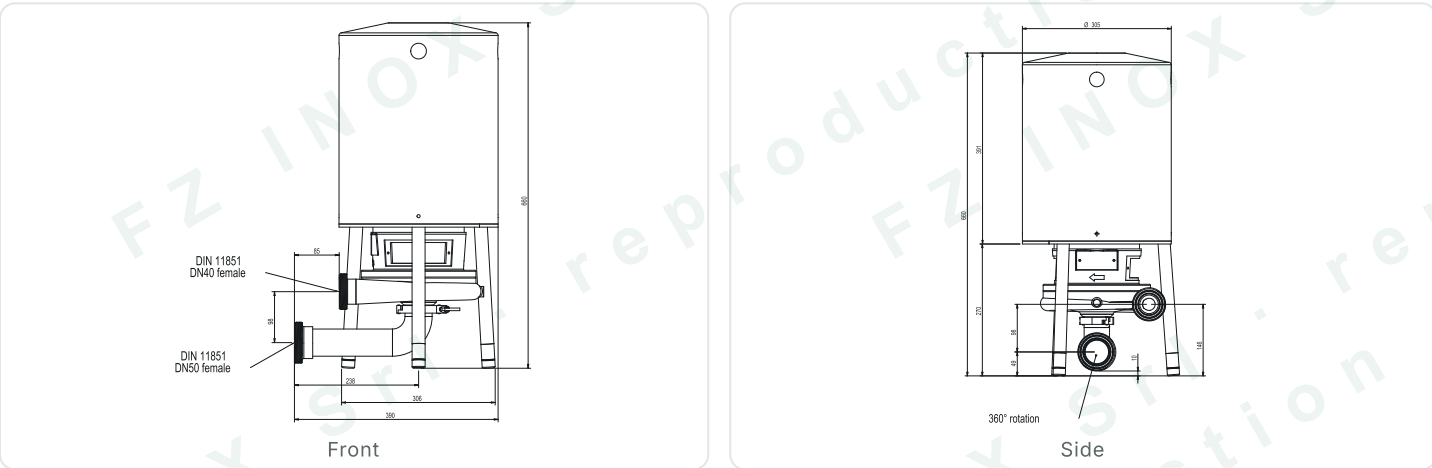
Overall dimensions in mm, 1.1 – 2.2 kW. Indicative, not binding.
