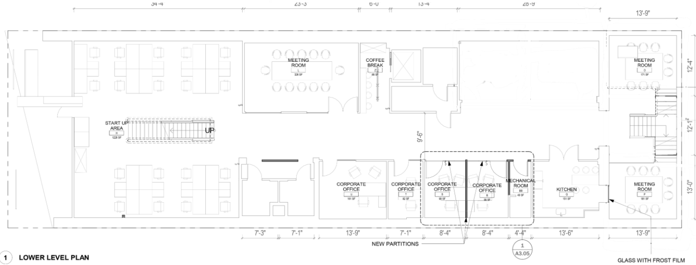
1 LOWER LEVEL PLAN
